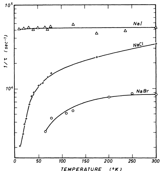
FIG. 4. Temperature dependence of 1/\tau(T) for the 3d^9 4s \rightarrow 3d^{10} transition in substitutional \text{Cu}^+ in NaCl, NaBr, and NaI.
