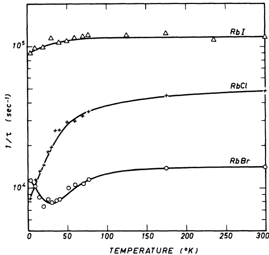
FIG. 2. Temperature dependence of 1/\tau(T) for the 3d^9 4s \rightarrow 3d^{10} transition in substitutional \text{Cu}^+ in \text{RbCl} , \text{RbBr} , and \text{RbI} .
