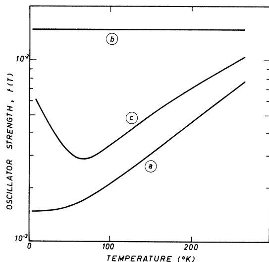
FIG. 1. Possible types of temperature dependence of the oscillator strength (schematic).
