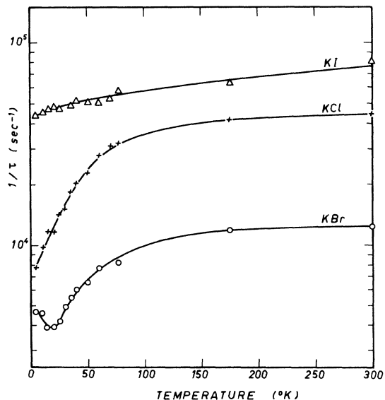
FIG. 3. Temperature dependence of 1/\tau(T) for the 3d^9 4s \rightarrow 3d^{10} transition in substitutional \text{Cu}^+ in \text{KCl} , \text{KBr} , and \text{KI} .
